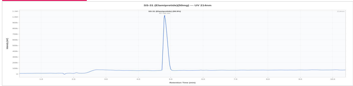
Representative chromatogram, Dedicated V0 (99.87% purity, closest to batch mean of 99.88%)
